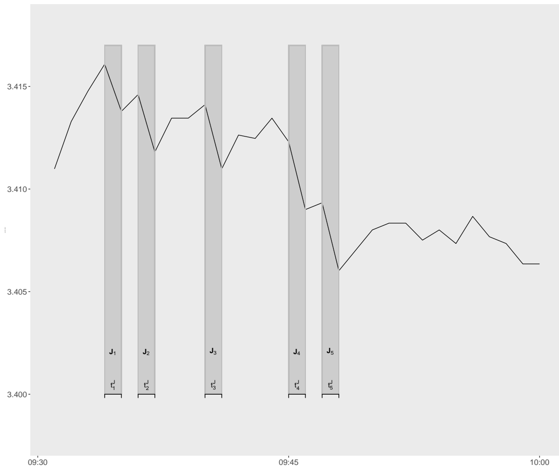
Figure 3.1: Return Decomposition
