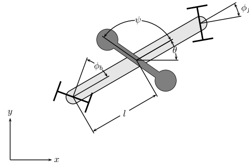
FIGURE 2. The simplified model of the Snakeboard
