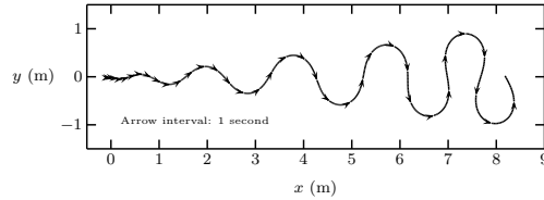
FIGURE 4. Position of the centre of mass for the (1,1,1) gait
