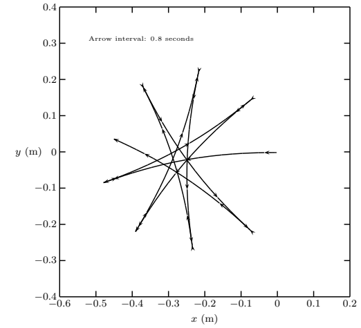
FIGURE 8. Position of the centre of mass for the (2, 1, 1) gait
