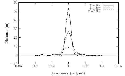
FIGURE 6. Distance traveled in the x -direction vs \omega_\psi for the (1,1,1) gait
